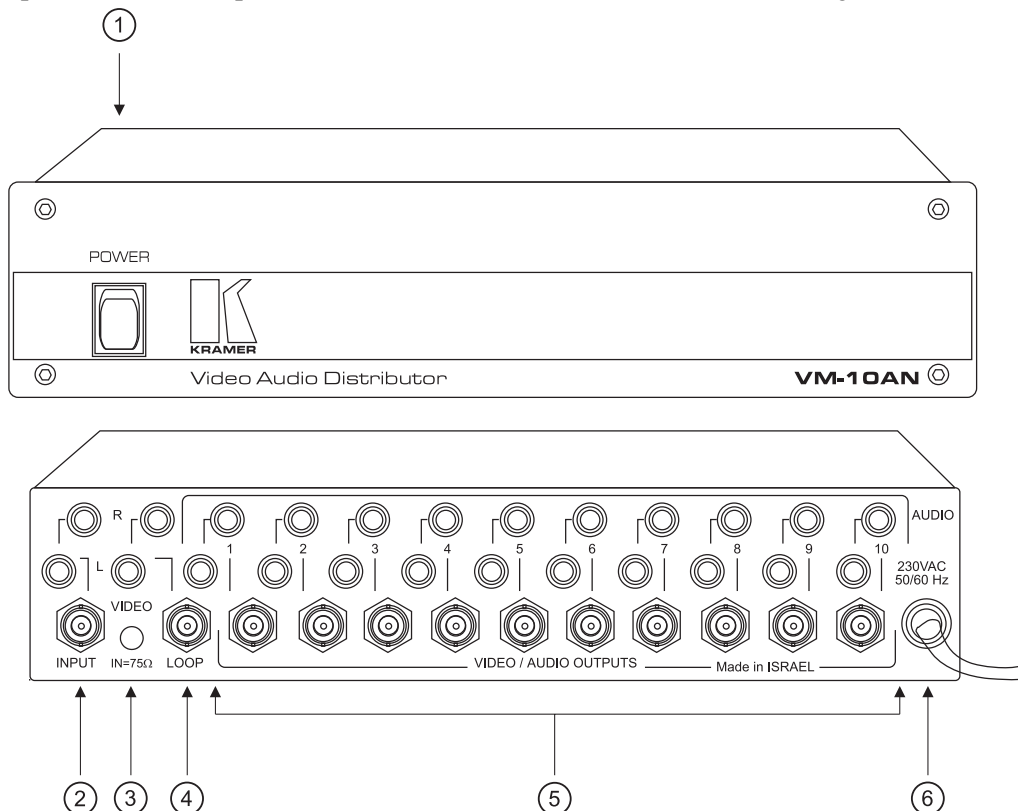
Figure 2: VM-10AN Front/Rear Panel Features
